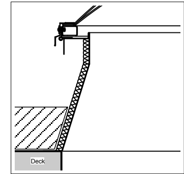
Tapered Kerb
